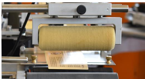
Soft foam roller for applying labels
